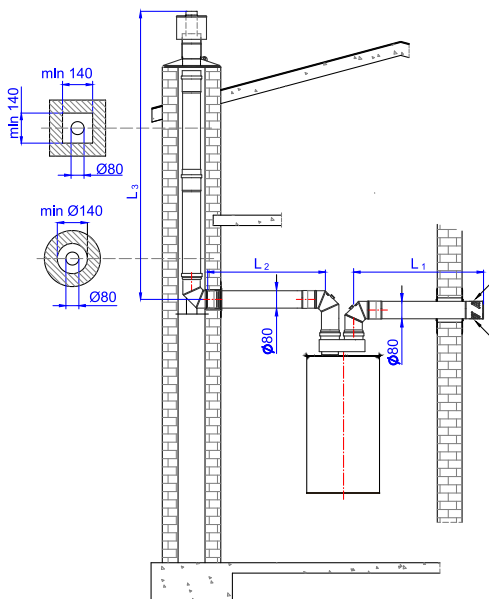
H_{\text{max}} = L_1 + L_2 + L_3 + (1\text{m}+1\text{m}+1\text{m}) \text{ (strata na kolankach)} rys. 3.8.3.2
