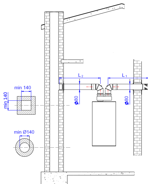
H = L_1 + L_2 + (1\text{m}+1\text{m}) \text{ (strata na kolankach)} rys. 3.8.4.1
