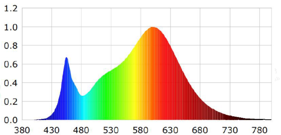
Spectral power distribution(3000K)
