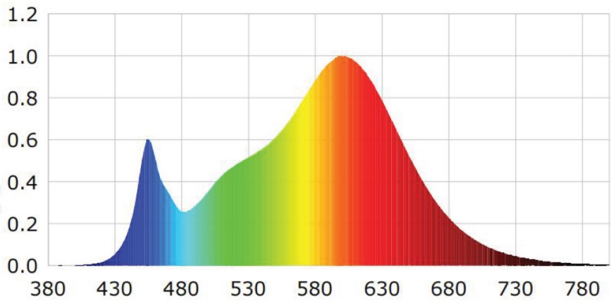
Spectral power distribution(3000K)
