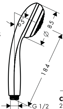
Crometta 85 1jet 28585000
